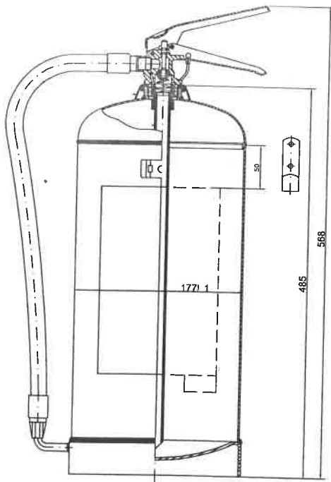
Cross-section
