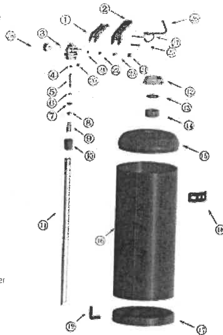
Expanded View
